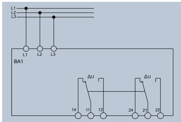
Fig. 3. Connection diagram
