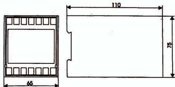
Fig. 2 : Dimensional drawing BUA1
