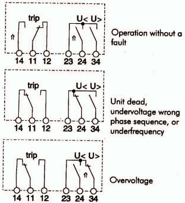
Fig. 4: Contact positions
