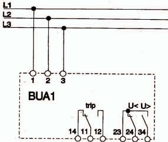
Fig. 3. Connection diagram
