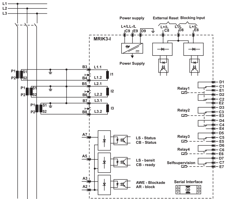
Figure 3.1 : Connections MARIK3-I
