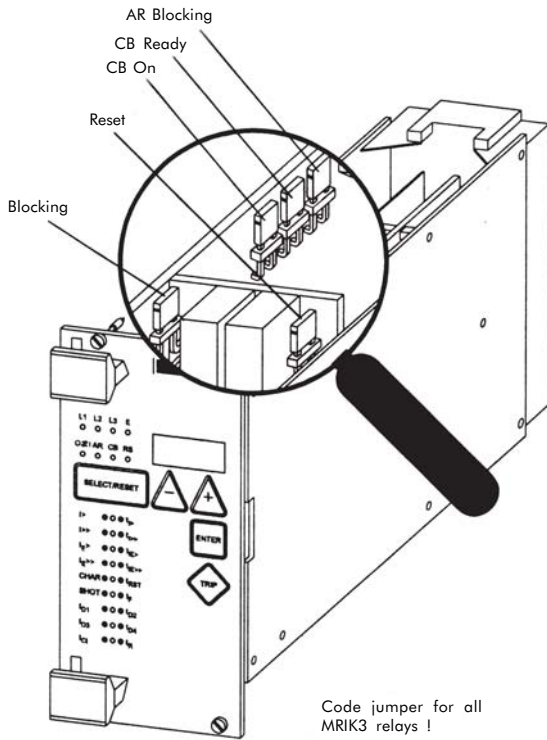
Fig. : 3.7 : Code jumper for MARIK3 relays
