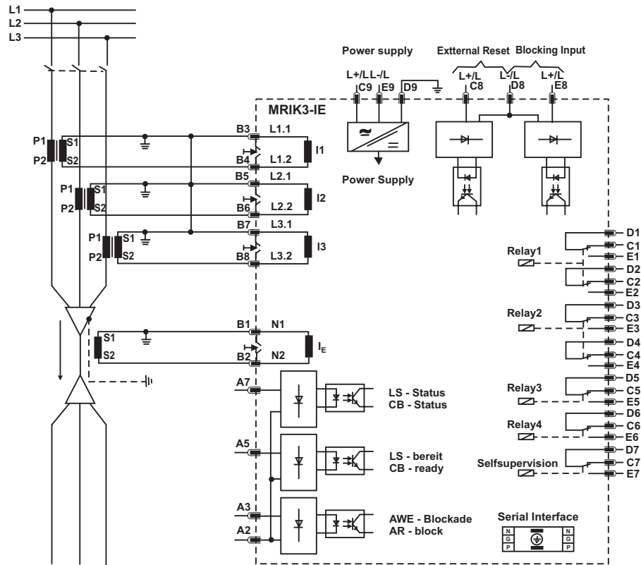
Figure 3.2 : Connections MARIK3-IE
