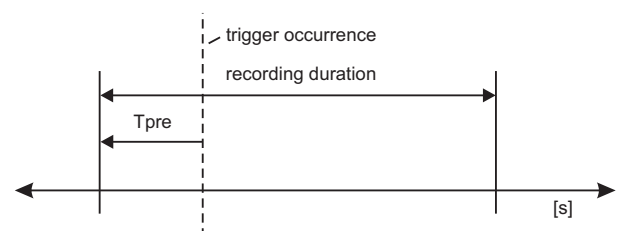
Fig. 3.4 : Basic set-up of the fault recorder
