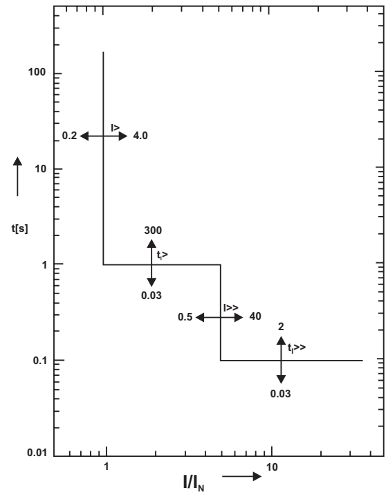
Fig. 7.7 : Definite time overcurrent Inverse
