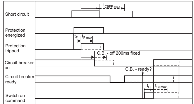
Fig. 4.4 : Unsuccessful AR
