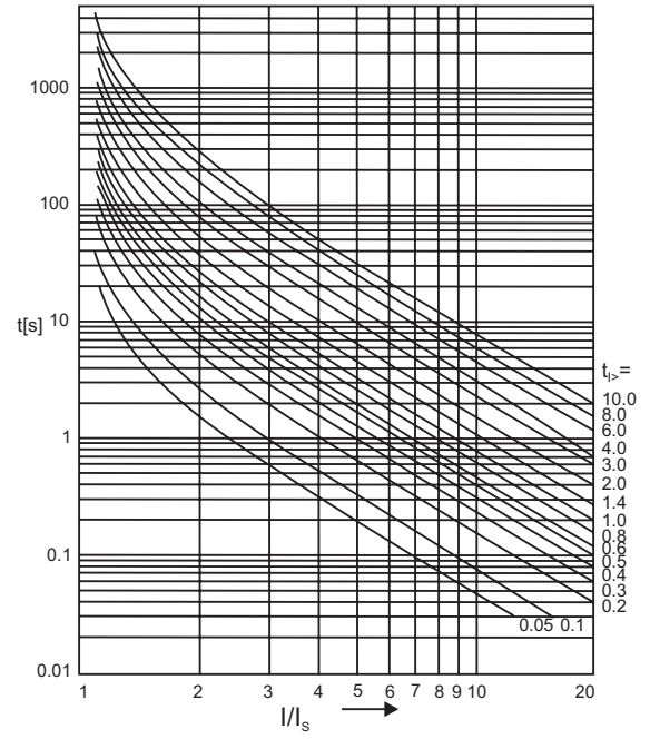
Fig. 7.3 : Extremely Inverse
