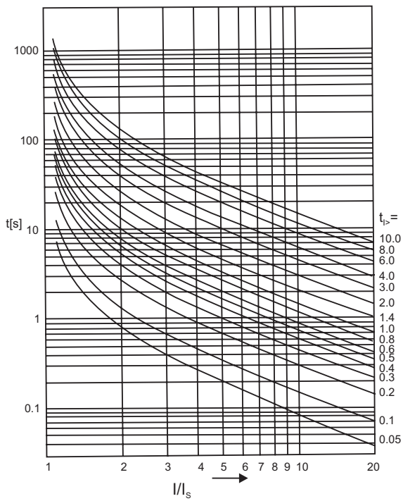
Fig. 7.2 : Very Inverse
