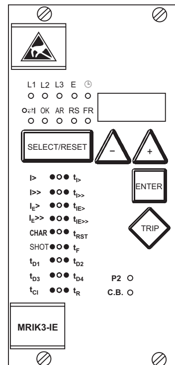
Fig. 3.6 : Front panel MRIK3-IE
