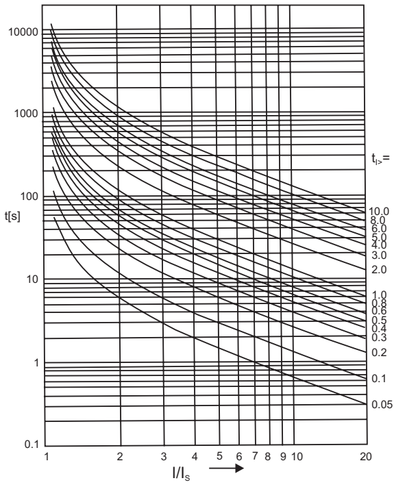
Fig. 7.5 : Long Time Inverse
