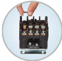
Easy access to blow-out & moving contacts
